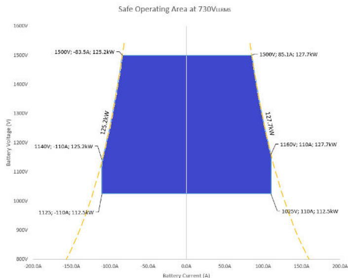
Figure 3: Safe Operating Area at 730V LL
