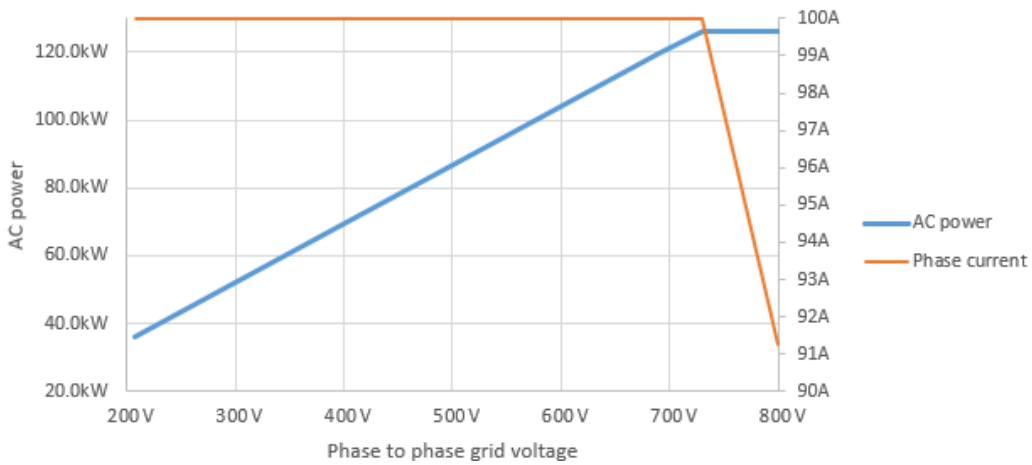
Figure 5: AC power vs AC phase to phase voltage
