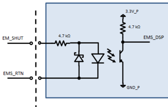
Figure 12 DSI input circuit
