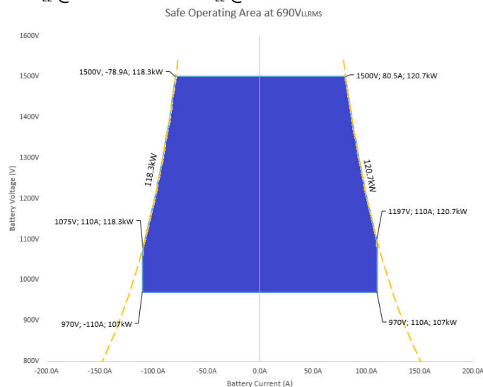
Figure 2: Safe Operating Area at 690V_{LL}
