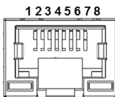
Figure 10 : CAN connector front view
