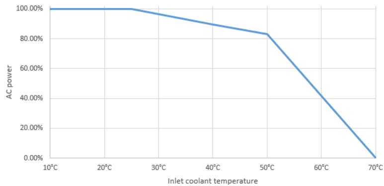
Figure 6: Maximum available AC power vs inlet coolant temperature
