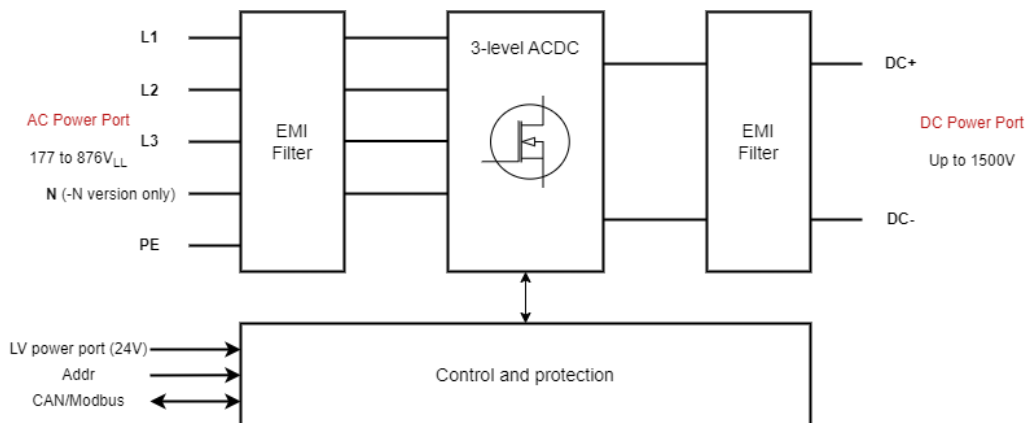
Figure 7: PCS high level synoptic
