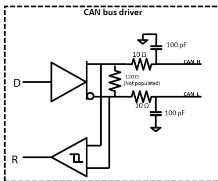
Figure 11: CAN transceiver simplified diagram
