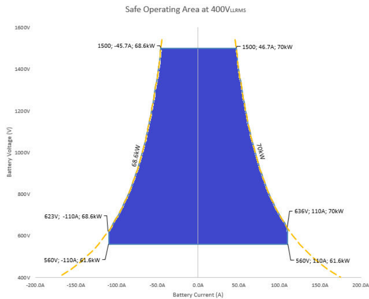
Figure 1: Safe Operating Area at 400V_{LL}
